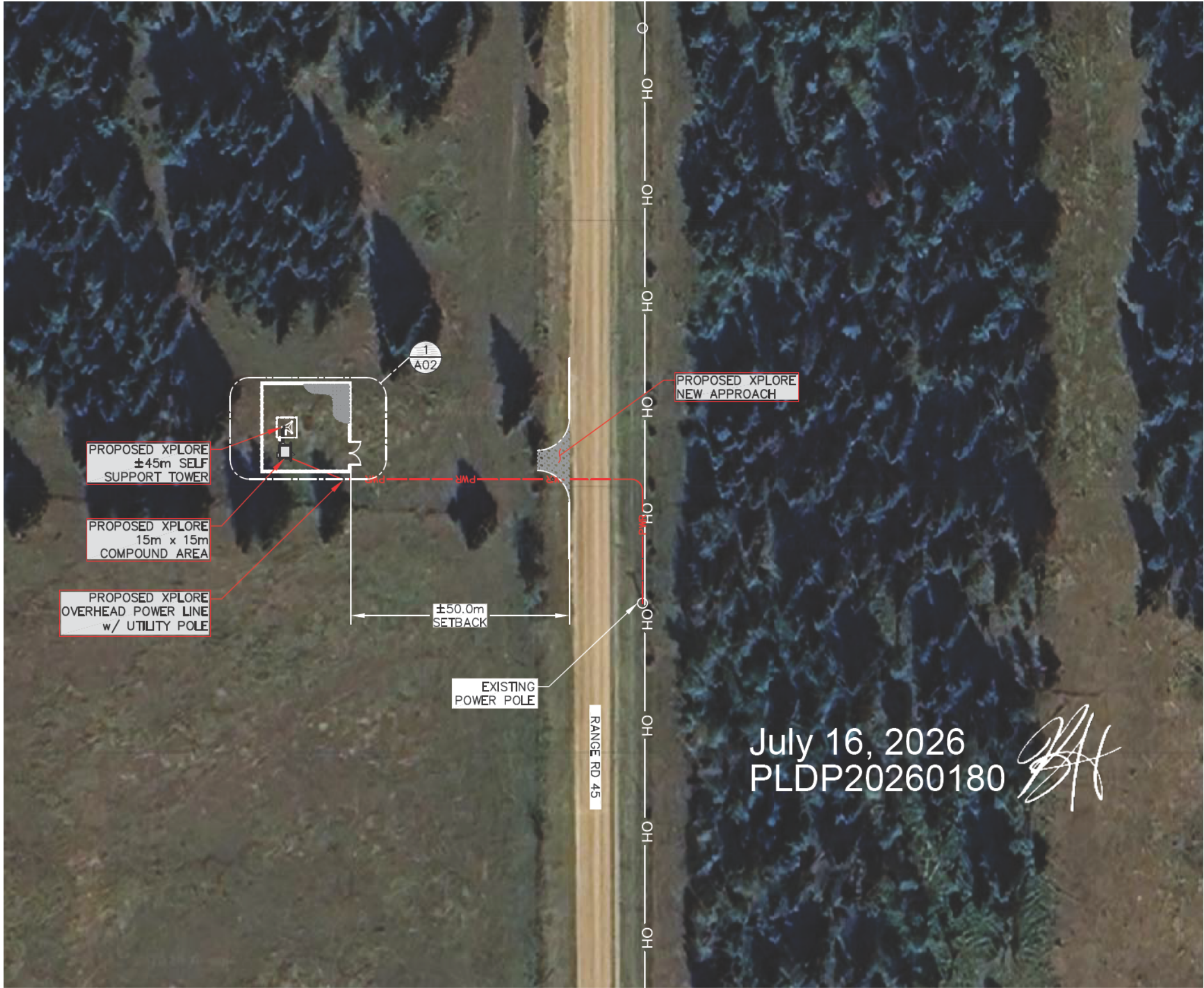
1 SITE PLAN
